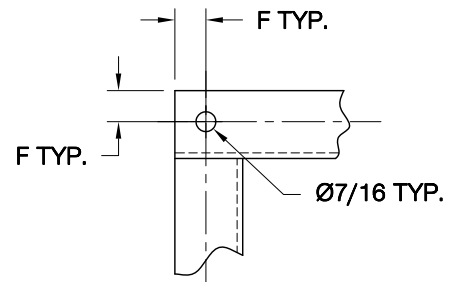
HOLE PATTERN DETAIL
